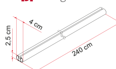
[3] Fixing-Bar Pro L
