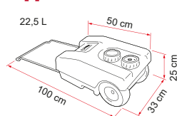
[1] Roll-Tank 23 F
