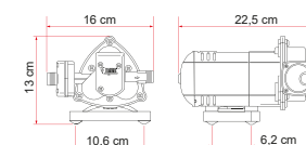
[3] Aqua 8 (7 & 10 litres)
